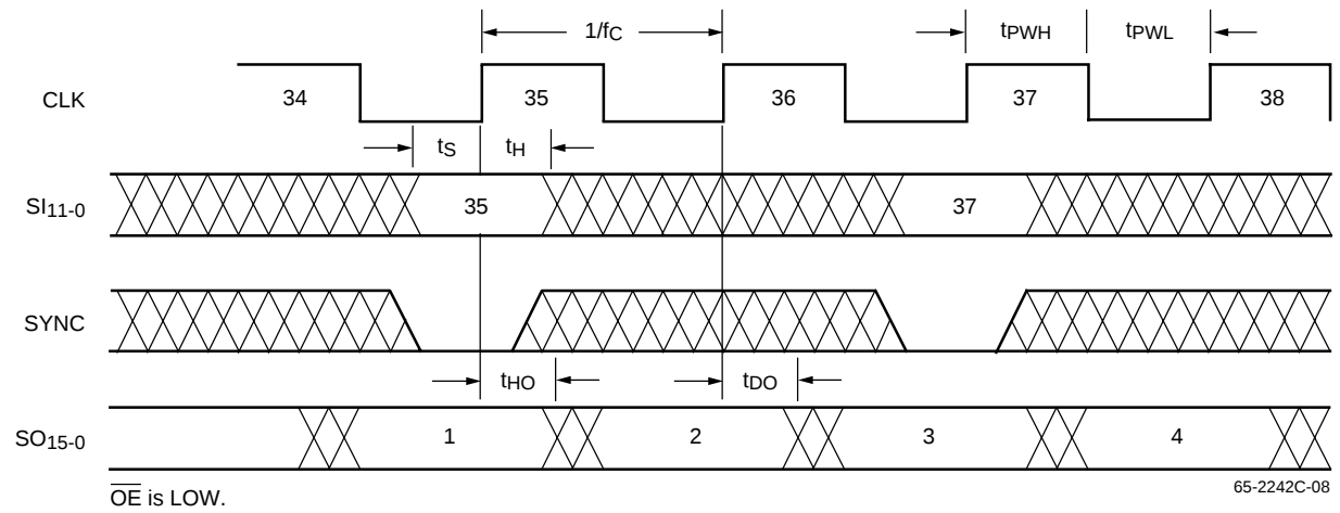
Figure 8. Interpolate Mode
