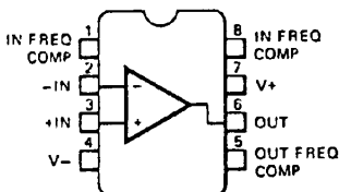
8-PIN MINI DIP (TOP VIEW) PACKAGE OUTLINE 9T PACKAGE CODE T
