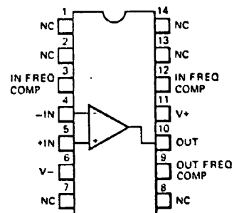
14-PIN DIP (TOP VIEW) PACKAGE OUTLINE 6A 9A PACKAGE CODE D P
