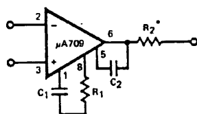
FREQUENCY COMPENSATION CIRCUIT
