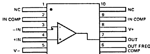
10-PIN FLATPAK (TOP VIEW) PACKAGE OUTLINE 3F PACKAGE CODE F
