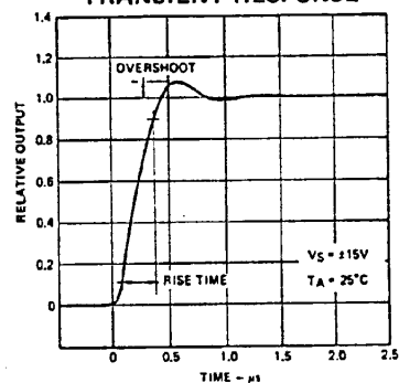
TRANSIENT RESPONSE
