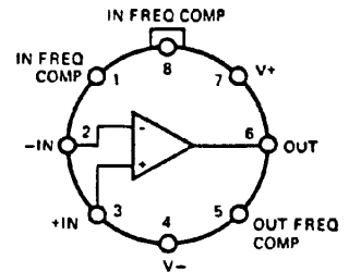
CONNECTION DIAGRAMS 8-PIN METAL CAN (TOP VIEW) PACKAGE OUTLINE 5S PACKAGE CODE H
