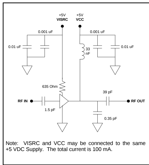
Schematic Including Off-Chip Components for 1800 - 2300 MHz
