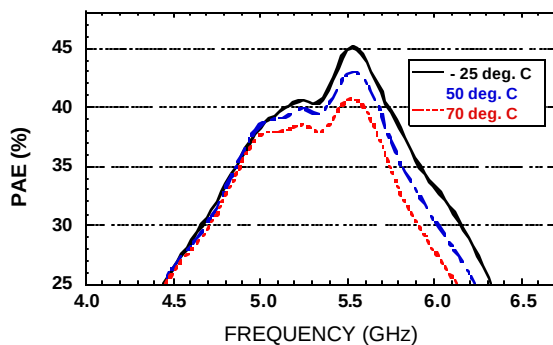
PAE Vs. Frequency
