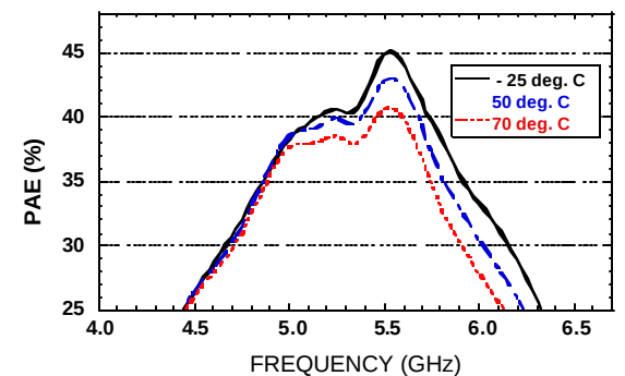
PAE Vs. Frequency
