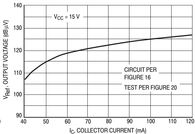
Figure 12. DIN 45004B versus Collector Current
