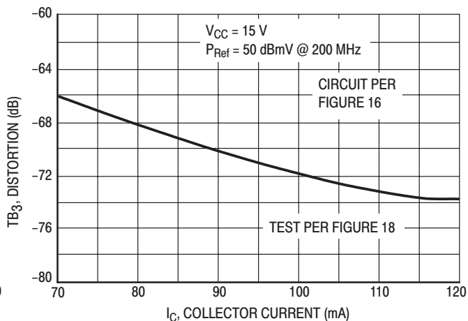
Figure 10. Triple Beat Distortion versus Collector Current
