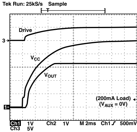
Figure 7. V_{CC} Cold start Power Up ( V_{AUX} = 0V )
