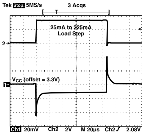
Figure 11. Load Transient (10% to 90%) Step Response
