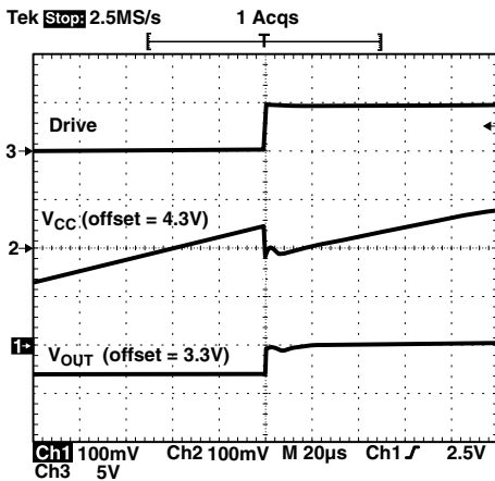
Figure 9. V_{CC} Power up ( V_{AUX} = 3.3V )
