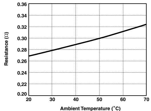
Figure 15. Switch Resistance vs Ambient Temperature
