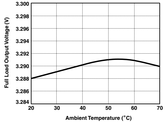
Figure 13. Regulator V_{OUT} vs T_{AMB} (250mA Load)
