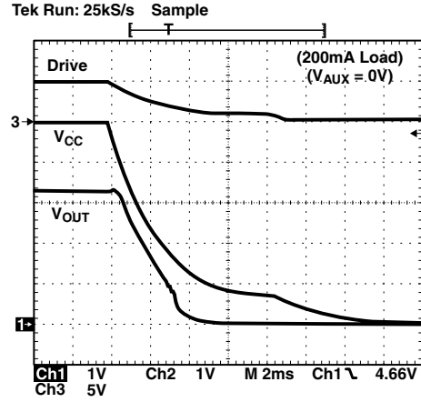
Figure 8. V_{CC} Complete Power Down ( V_{AUX} = 0V )
