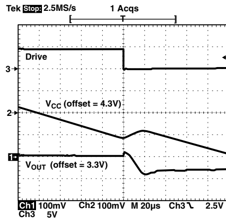
Figure 10. V_{CC} Power Down ( V_{AUX} = 3.3V )
