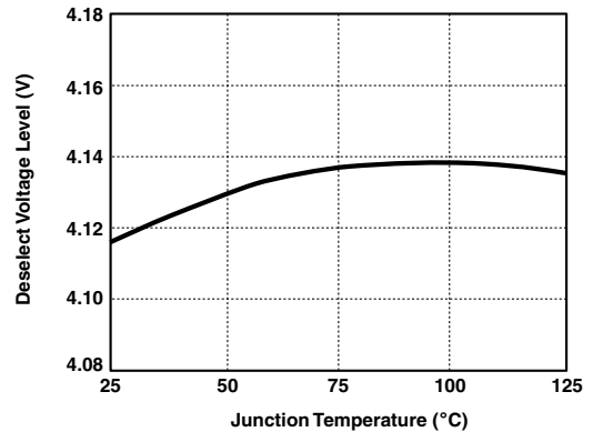
Figure 14. Deselect Threshold vs T_{JUNCT}
