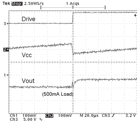
Figure 6. V CC Power-up (V AUX = 3.3V).
