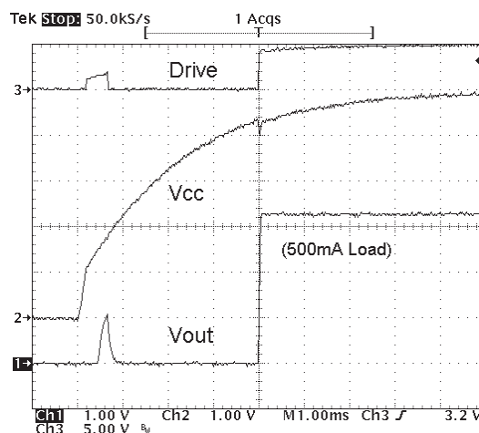
Figure 5. V CC Power-up Cold Start.
