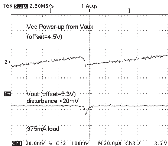
Fig 2.9 V_{CC} power up ( V_{AUX} = 3.3V )
