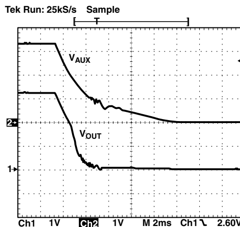
Figure 16. V_{AUX} Full Power Down (Load = 400mA)
