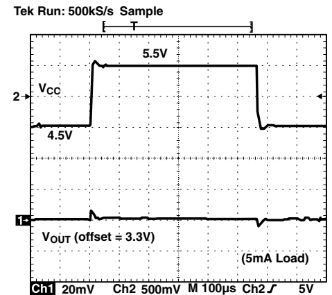
Figure 22. Line Transient ( 1V_{pp} ) Response
