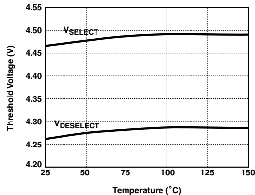
Figure 24. Select/Deselect Threshold Variation with T_{JUNC}
