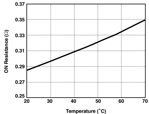
Figure 25. V_{AUX} Switch Resistance vs T_{AMB}
