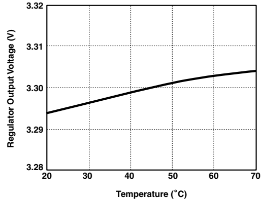
Figure 23. V_{OUT} Variation with T_{AMB} (400mA Load) T
