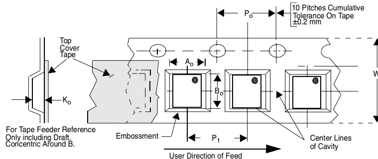
Figure 11. Tape and Reel Mechanical Data
