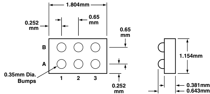
PACDN1404C
