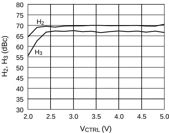
AS193-73 Harmonics vs. Control Voltage P IN = 34.5 dBm, 900 MHz, GSM Pulsed
