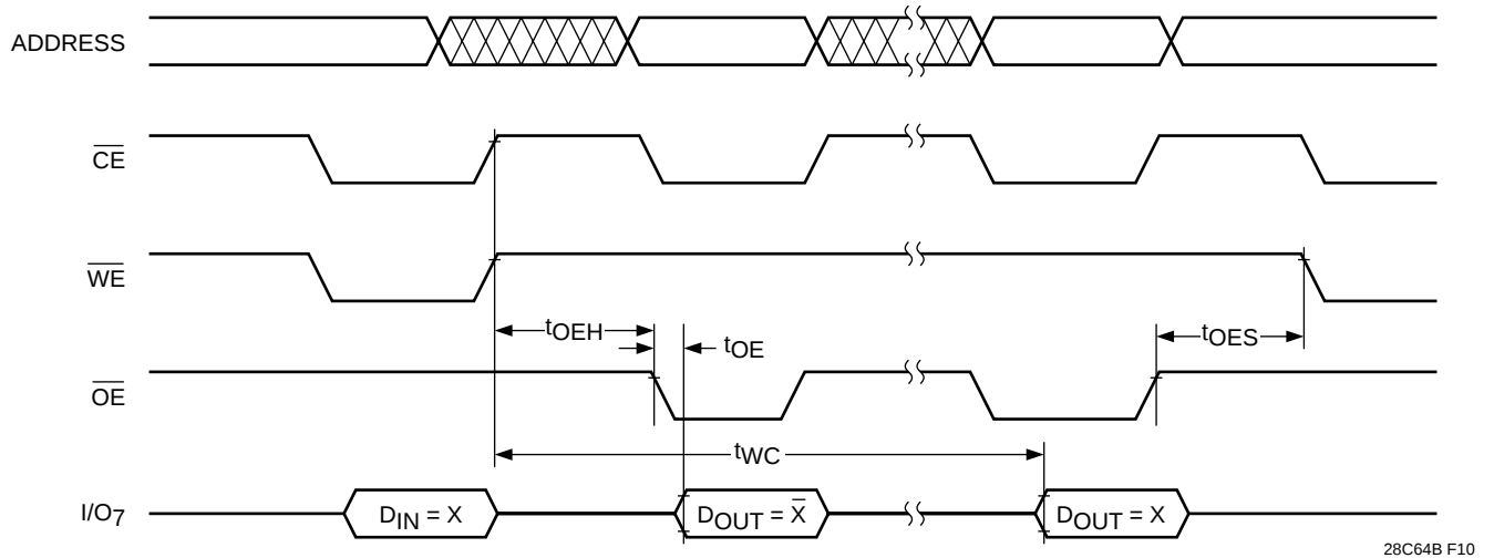
Figure 7. \overline{\text{DATA}} Polling
