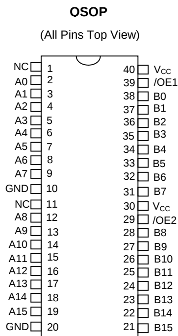
Figure 2. Pin Configuration
