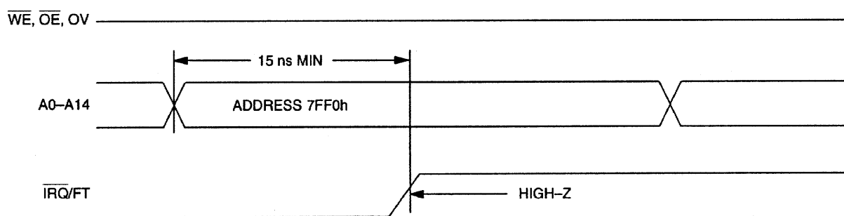
CLEARING IRQ WAVEFORMS Figure 3
