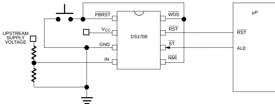
PUSH-BUTTON RESET CONTROLLED BY \overline{\text{NMI}} AND \overline{\text{WDS}} Figure 3
