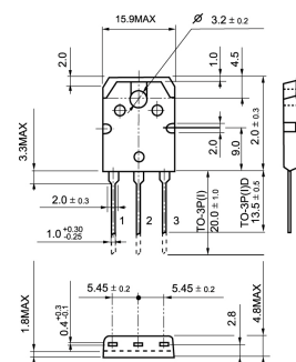
TO-3P(I)D
