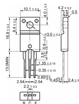
TO-220F
