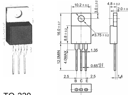
TO-220
