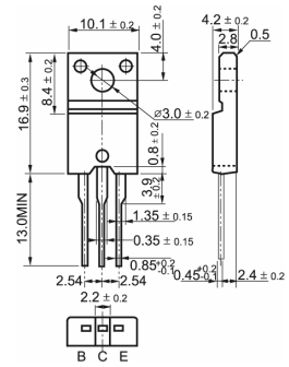
TO-220F
