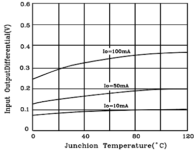
Dropout Voltage
