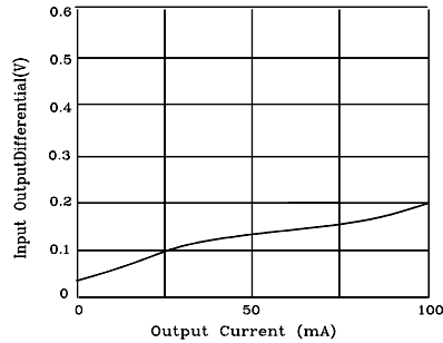
Dropout Voltage
