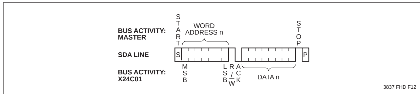
Figure 7. Byte Read
