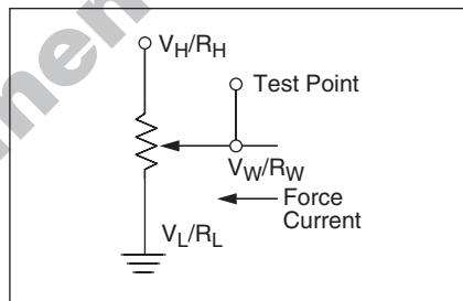
Test Circuit #2
