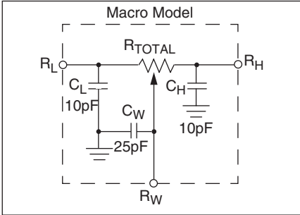
Test Circuit #3
