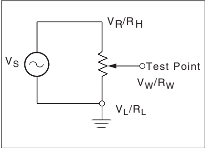
Test Circuit #1
