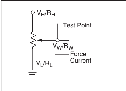
Test Circuit #2
