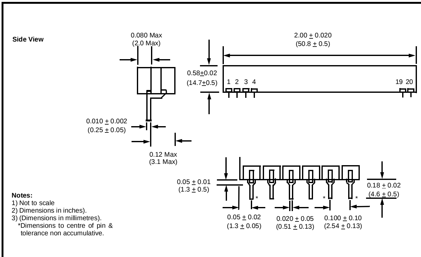
Figure 9 - Mechanical Data
