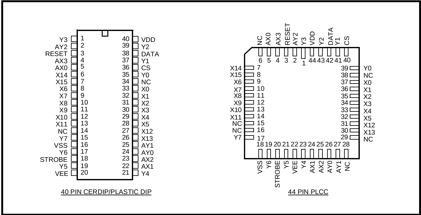
Figure 2 - Pin Connections
