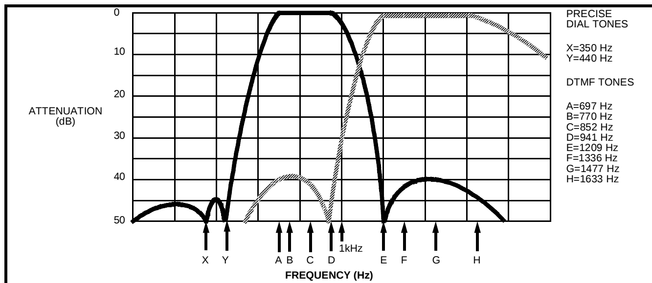
Figure 3 - Filter Response
