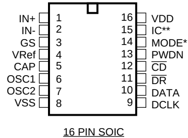
Figure 2 - Pin Connections
