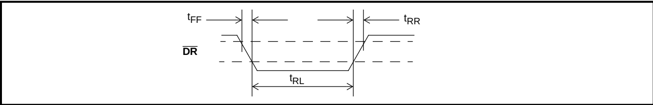
Figure 9 - \overline{DR} Output Timing (Mode 0)
