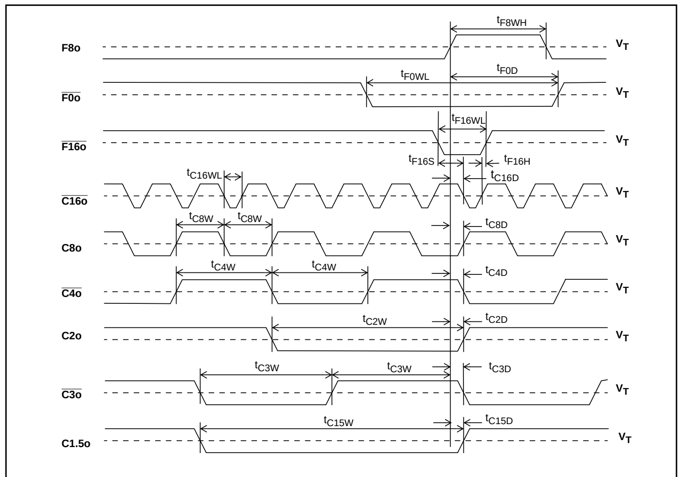
Figure 20 - Output Timing 1
