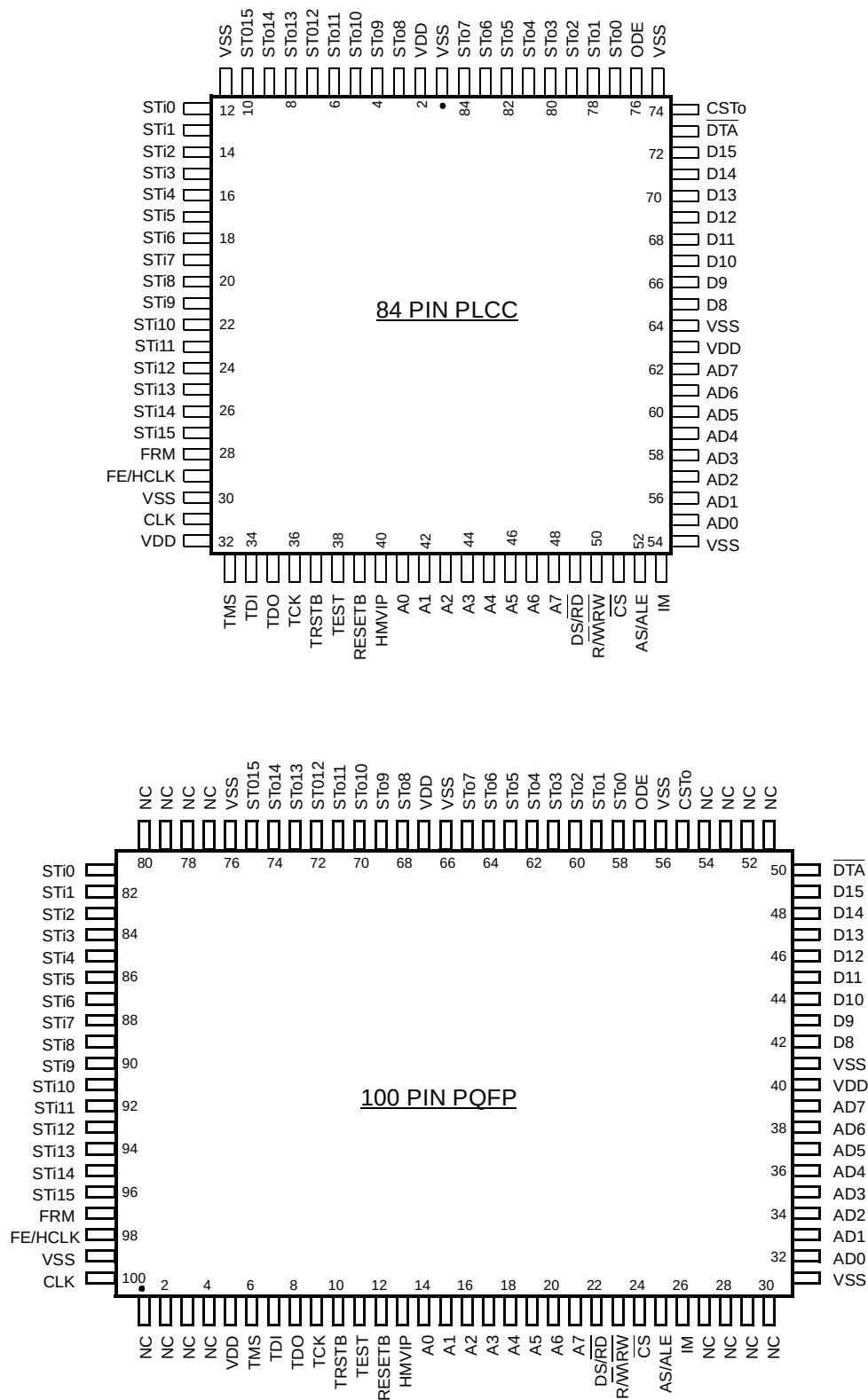
Figure 2 - Pin Connections
