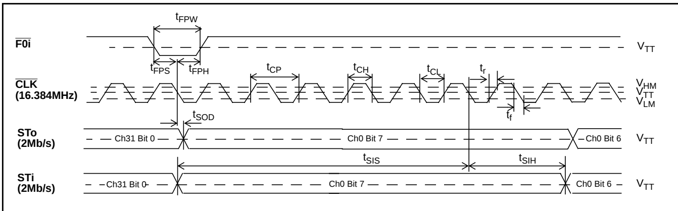
Figure 10 - ST-BUS Timing for Stream rate of 2.048 Mb/s when \overline{\text{CLK}} = 16.384\text{MHz}
