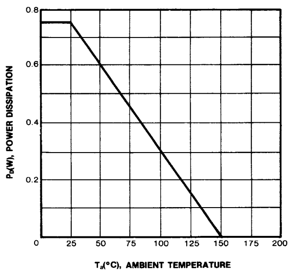
POWER DERATING
