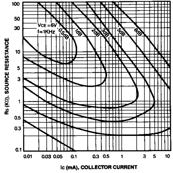
NOISE FIGURE
