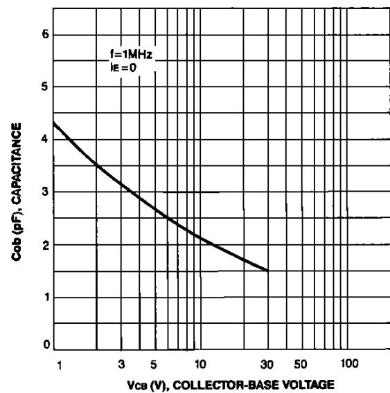
OUTPUT CAPACITANCE
