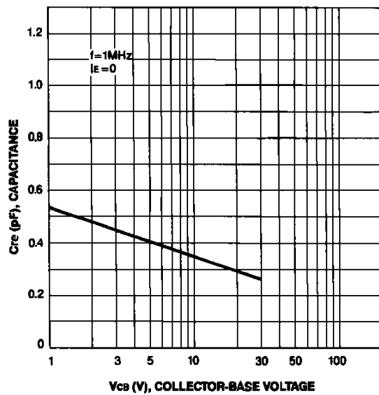
REVERSE CAPACITANCE
