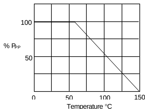
Figure 4 - Derating Curve
