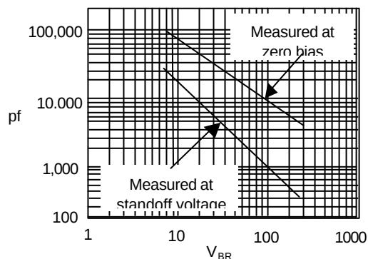
Figure 3 - Typical Capacitance
