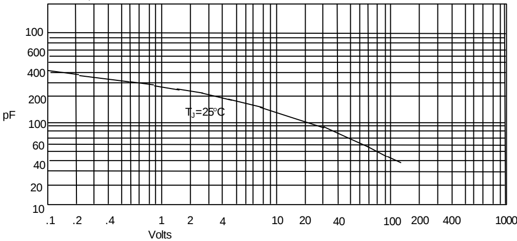
Figure 3 Junction Capacitance
