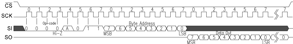
Figure 9 Memory Read
