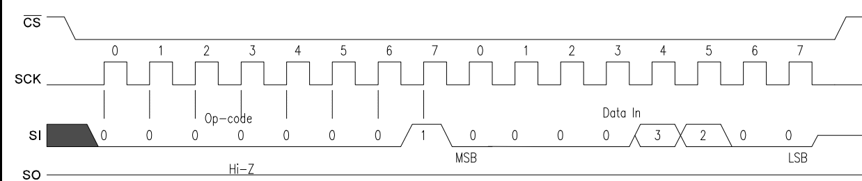
Figure 7. WRSR Bus Configuration
