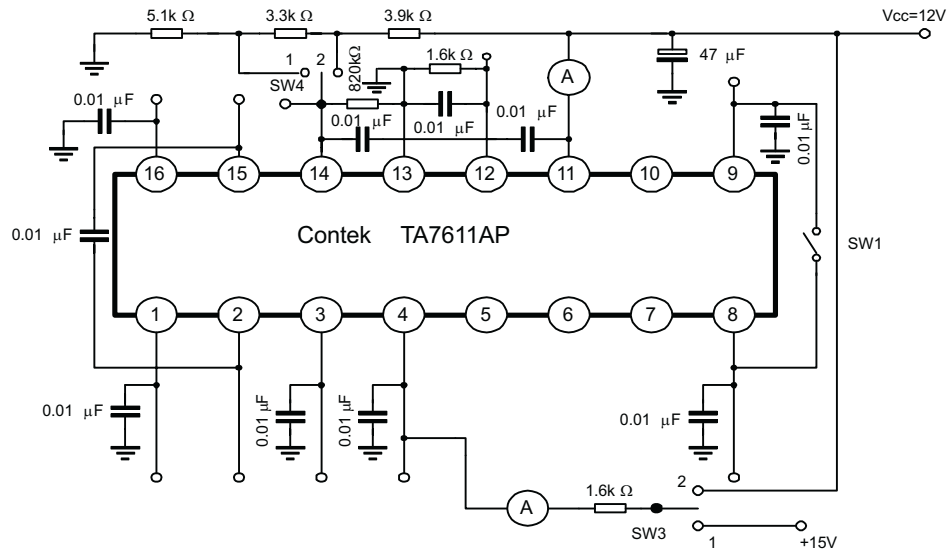
TEST CIRCUIT 2
