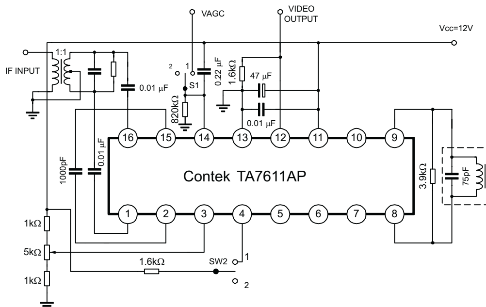
TEST CIRCUIT 2
