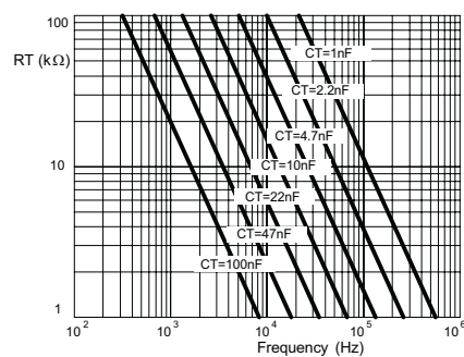
\tau(R_T > 5k\Omega) Timing Resistance Vs Frequency
