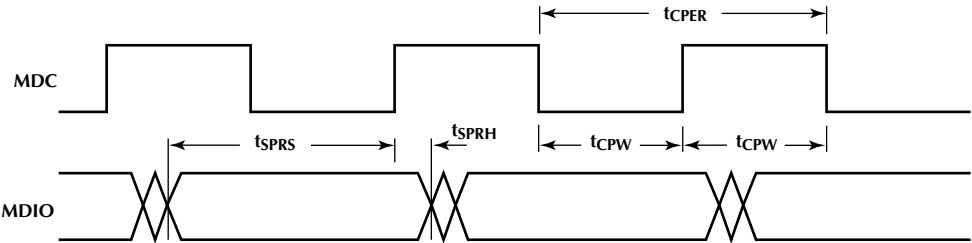
Figure 4. MII Management Interface Read Timing
