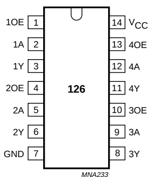
Fig.1 Pin configuration.
