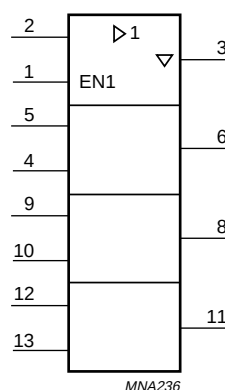
Fig.4 IEC logic symbol.
