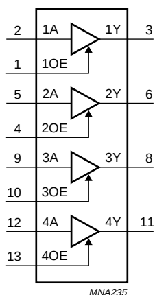
Fig.3 Functional diagram.
