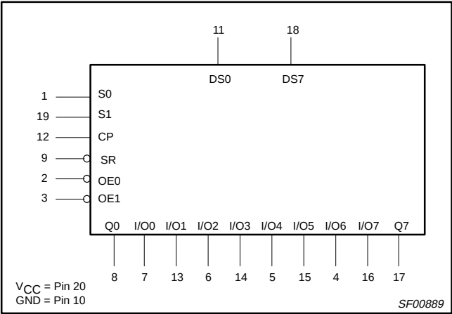
LOGIC SYMBOL
