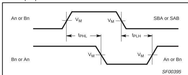
Waveform 2. Propagation Delay, An to Bn or Bn to An and SBA to An or SAB to Bn
