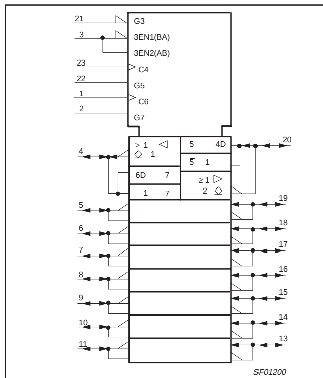
LOGIC SYMBOL – 74F648
