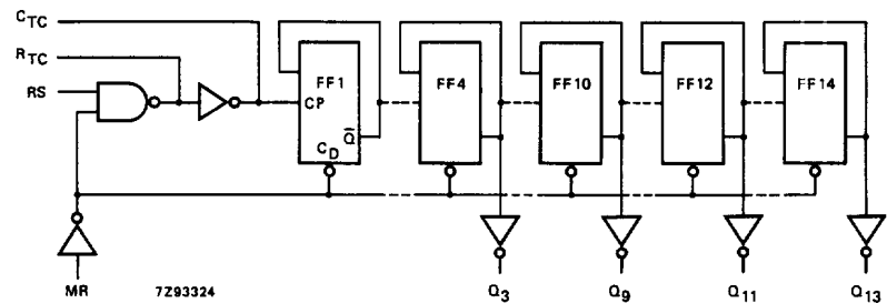
Fig.5 Logic diagram.
