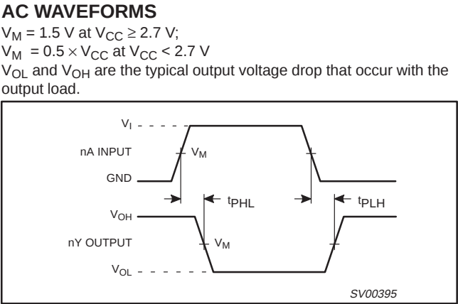
Figure 6. Input (nA) to output (nY) propagation delays.
