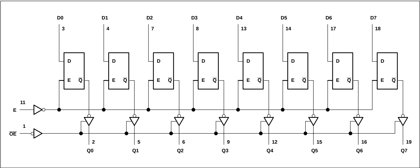
LOGIC DIAGRAM
