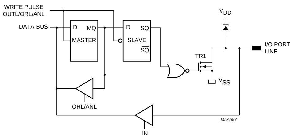
Fig.16 Open drain type I/O (Option 2).
