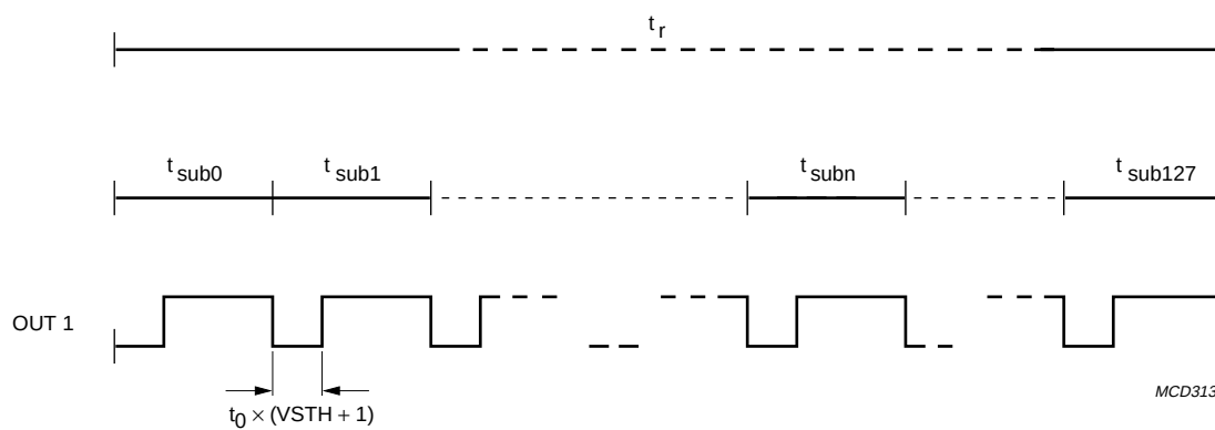
Fig.11 Coarse adjustment output (OUT1).
