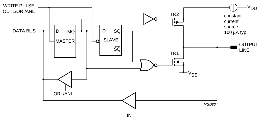
Fig.17 Push-pull type output (Option 3).
