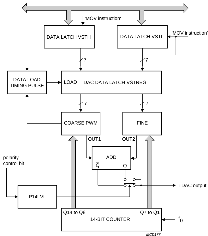
Fig.10 Block diagram of the 14-bit PWM DAC.
