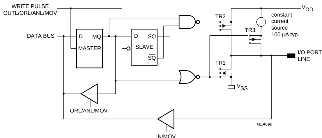
Fig.15 Standard output with switched pull-up current source (Option 1).
