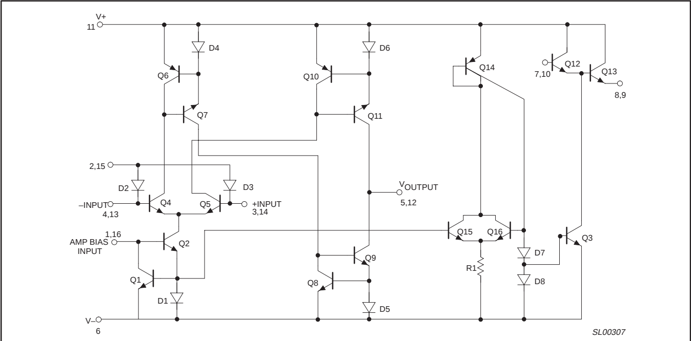
Figure 2. Circuit Schematic
