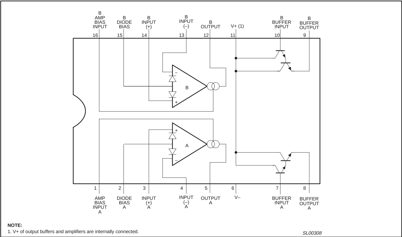
Figure 3. Connection Diagram
